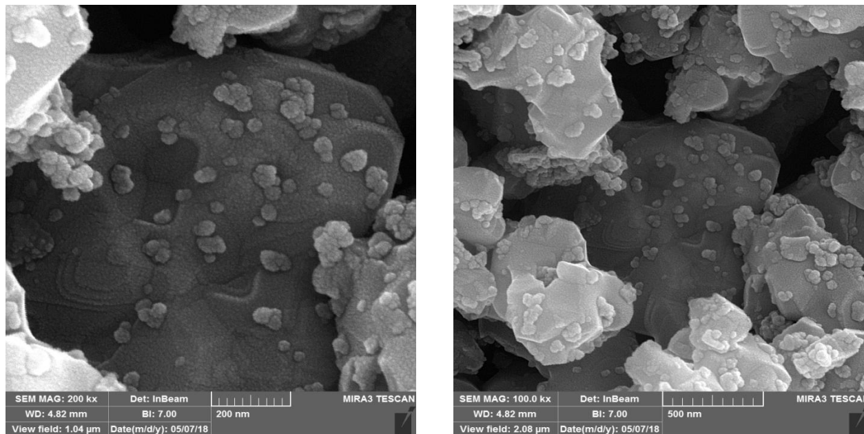
Fig. 3 SEM images for TiO 2 NPs for rutile phase.
