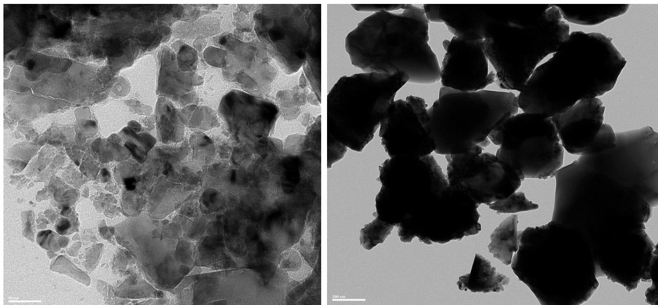
Fig. 5 TEM images of rutile phase for TiO 2 NPs
