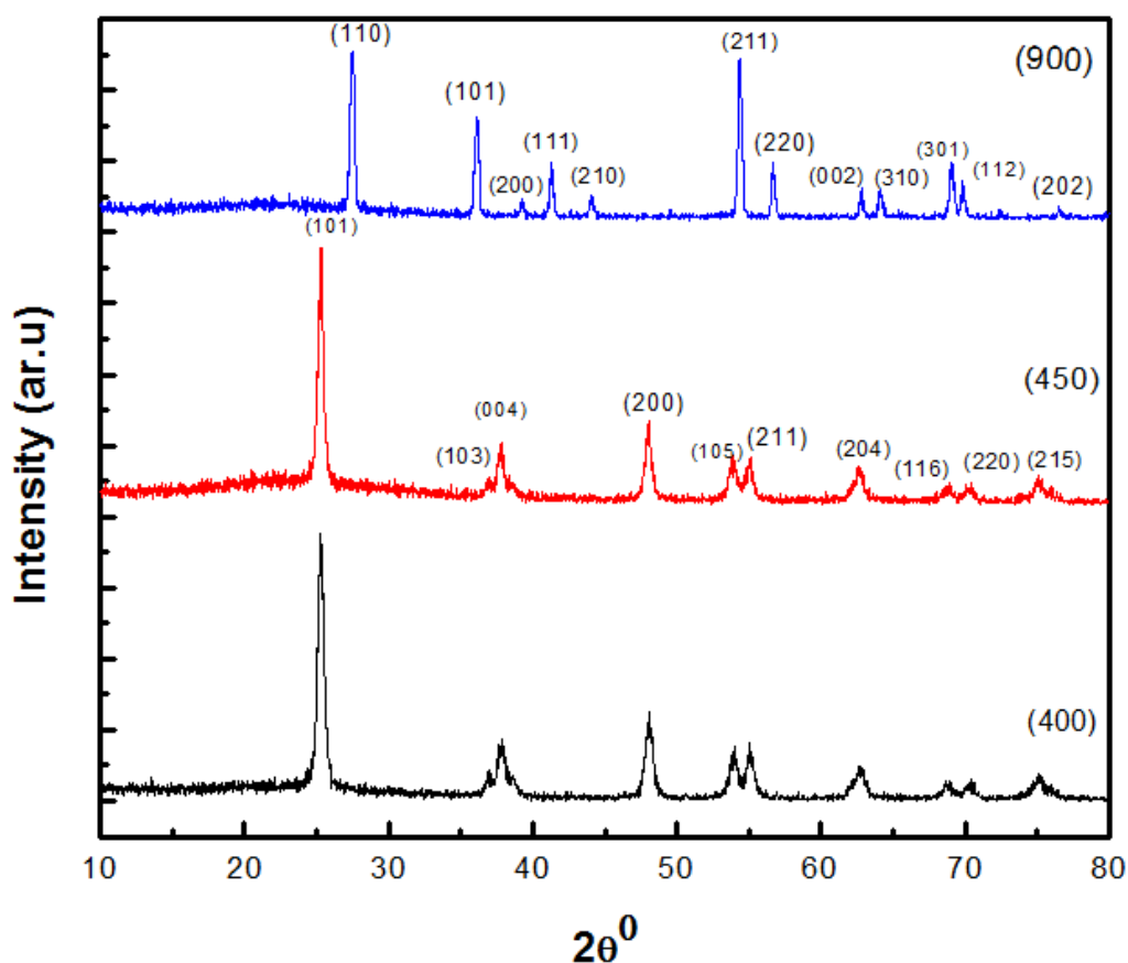
Fig. 1: XRD pattern Anatase & Rutile phases at different temperatures (400, 450, and 900) °C.
