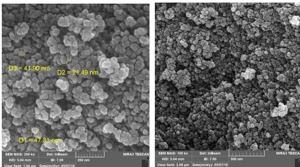
Fig. 2 FESEM images of \text{TiO}_2 NPs for anatase phase .
